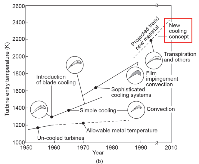
Fig. 4. The use of AD/AM for a better cooling structure of a high-pressure turbine blade [1]. (a) Different cooling mechanisms; (b) development of turbine blade cooling structure.
