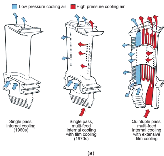
Fig. 4. The use of AD/AM for a better cooling structure of a high-pressure turbine blade [1]. (a) Different cooling mechanisms; (b) development of turbine blade cooling structure.
